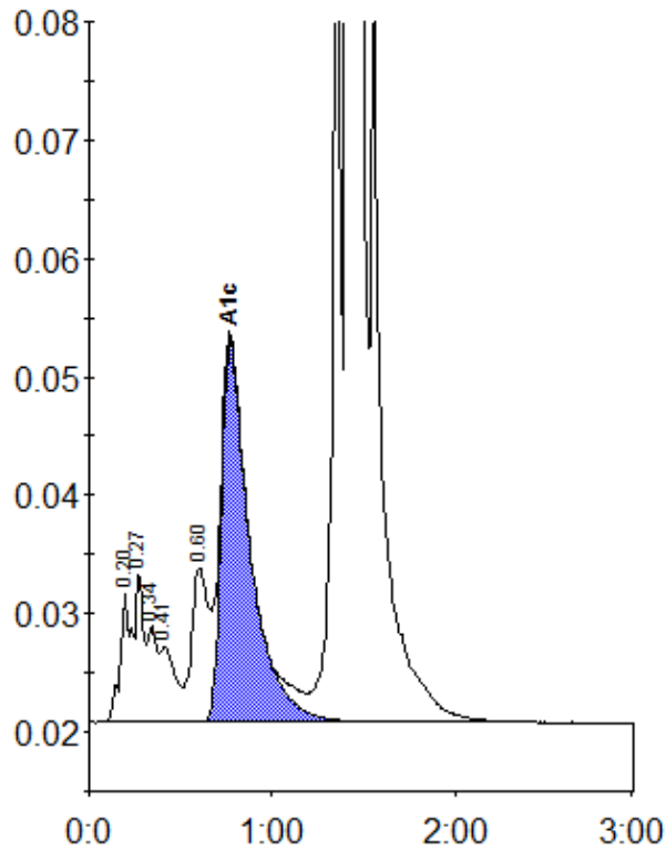
Peak table - ID: 10265225
