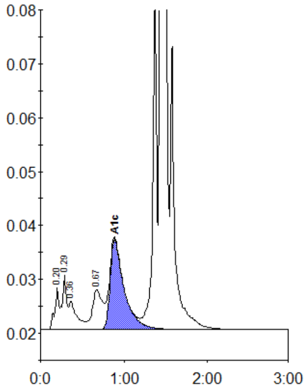
Peak table - ID: 10265263
