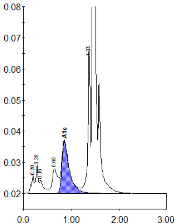
Peak table - ID: 10297925
