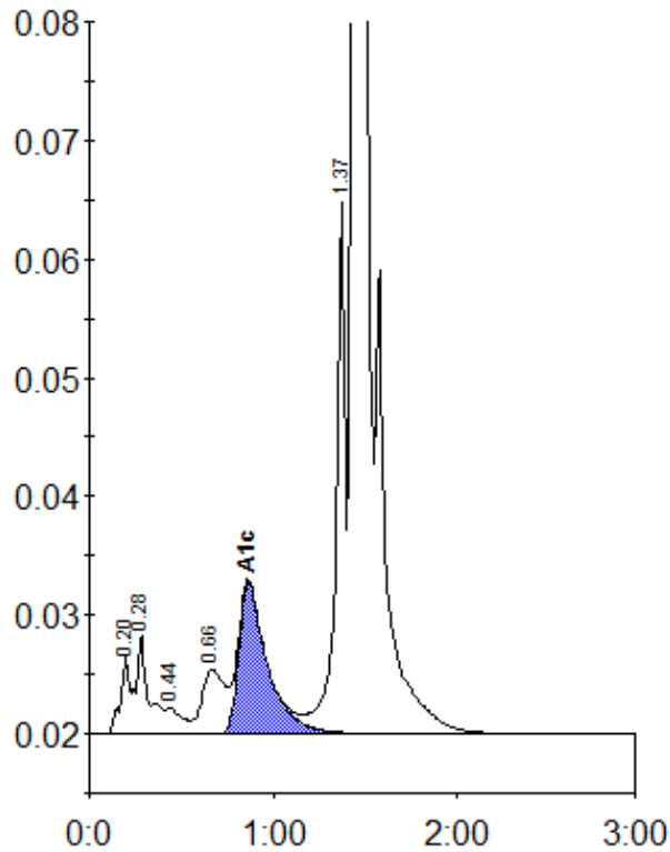
Peak table - ID: 10214694
