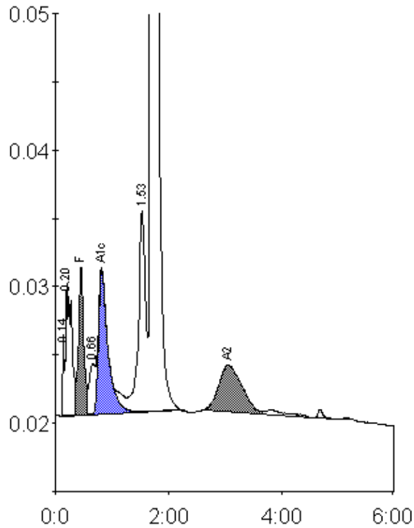
Peak table - ID: 10265997
