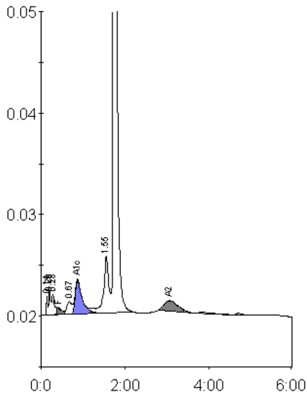
Peak table - ID: 10279447
