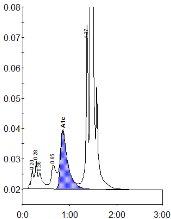
Peak table - ID: 10297544
