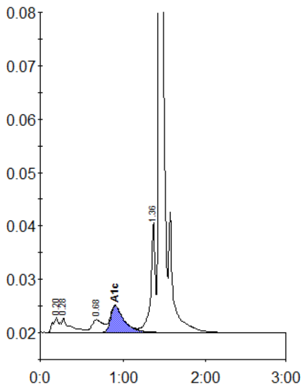
Peak table - ID: 10209703
