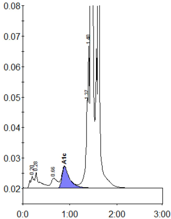
Peak table - ID: 10303519
