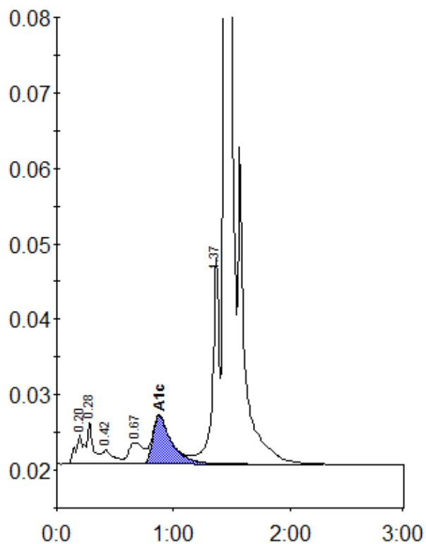
Peak table - ID: 10278463
