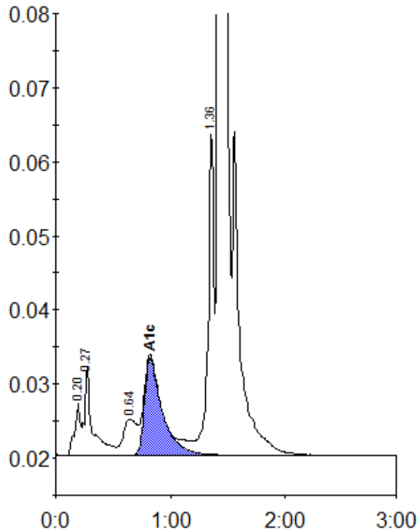
Peak table - ID: 10304728
