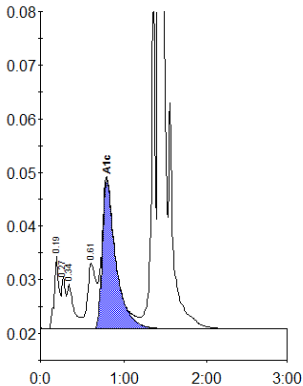
Peak table - ID: 10293050
