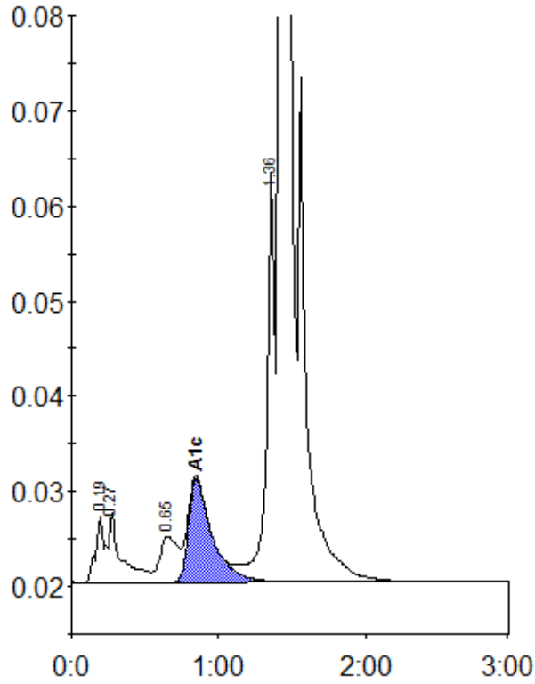
Peak table - ID: 10325414
