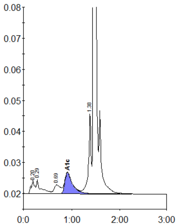
Peak table - ID: 10325890
