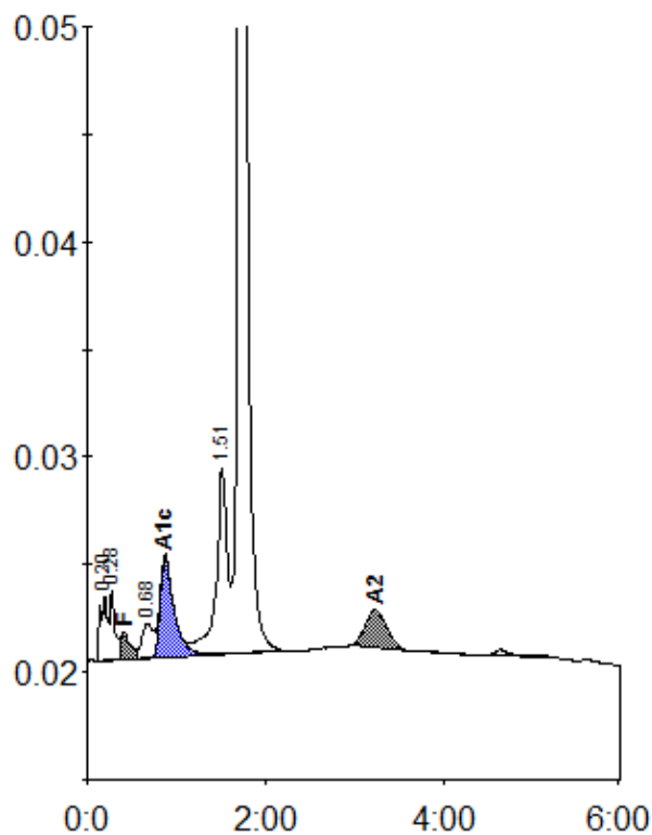
Peak table - ID: 10171326
