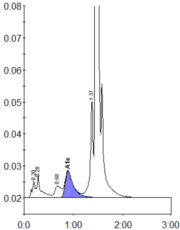
Peak table - ID: 10224158
