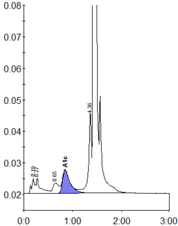
Peak table - ID: 10321986
