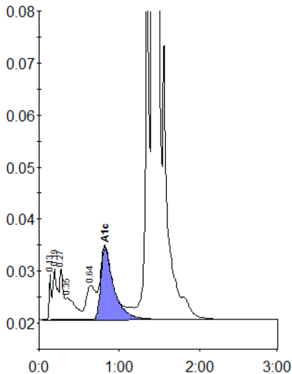
Peak table - ID: 10318785
