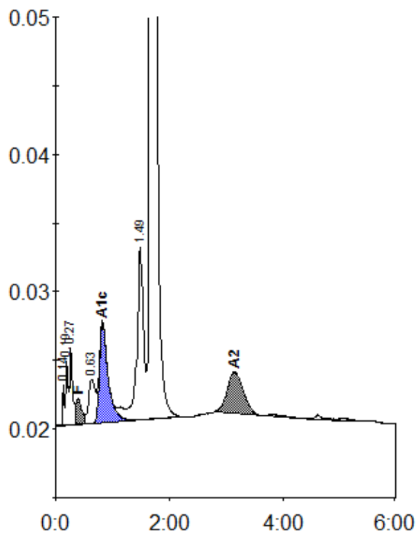
Peak table - ID: 10329394
