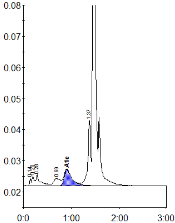
Peak table - ID: 10299128
