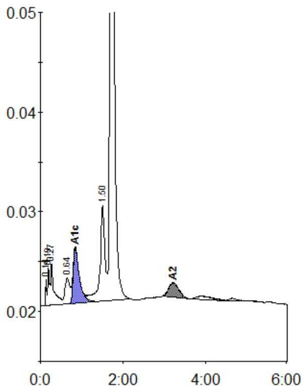
Peak table - ID: 10224743
