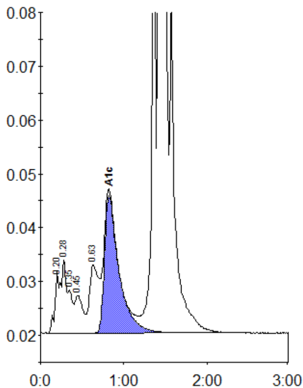
Peak table - ID: 10324583
