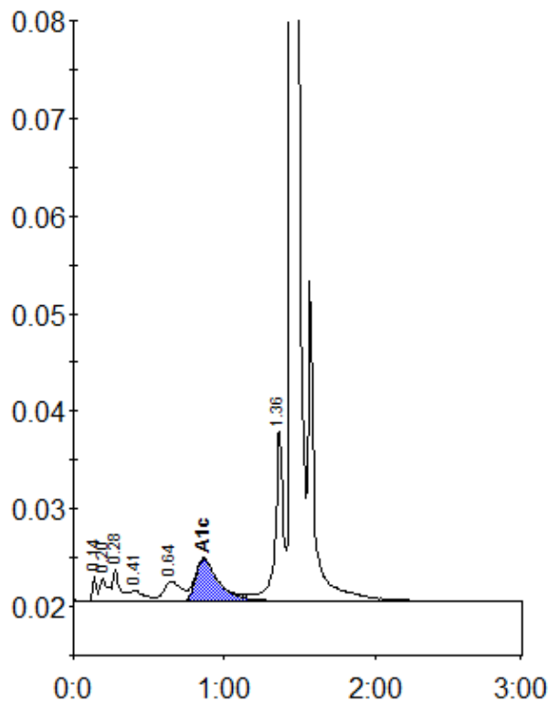
Peak table - ID: 10204192
