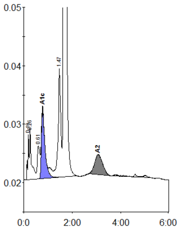
Peak table - ID: 10299522
