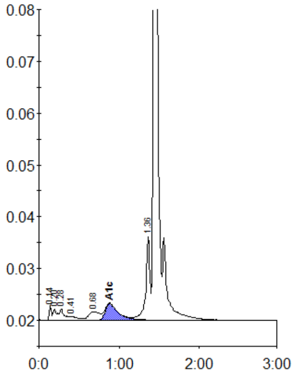
Peak table - ID: 10208227
