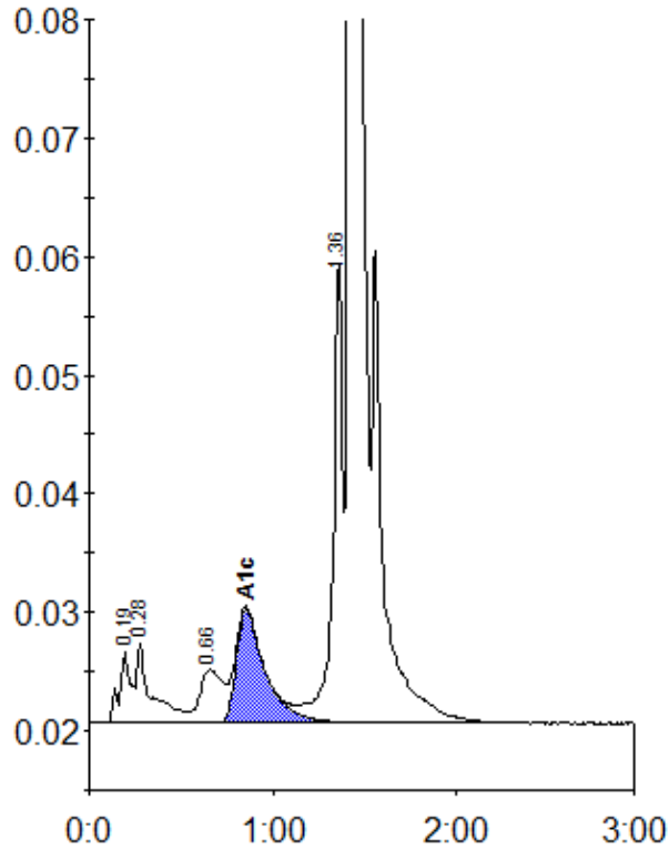
Peak table - ID: 10176924
