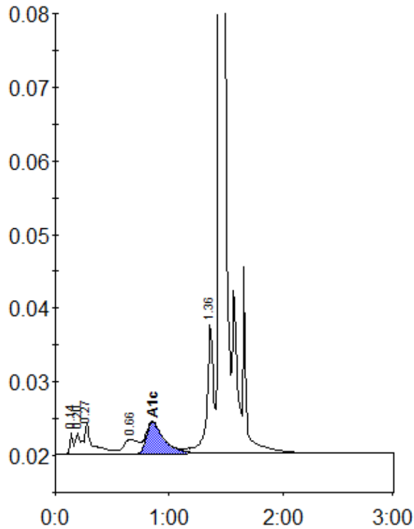
Peak table - ID: 10314698
