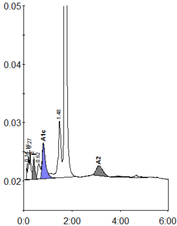
Peak table - ID: 10210982
