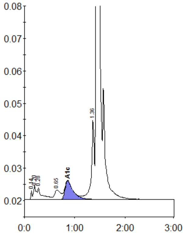
Peak table - ID: 10213203
