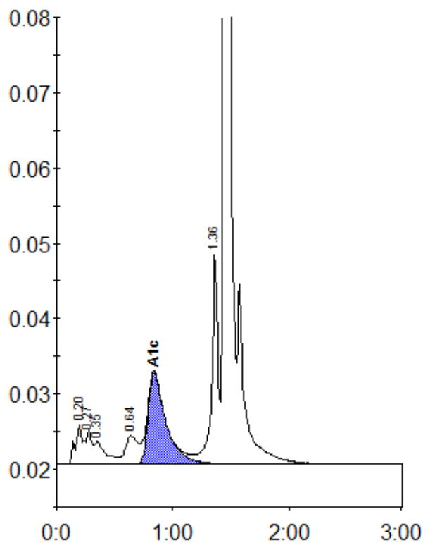
Peak table - ID: 10209635
