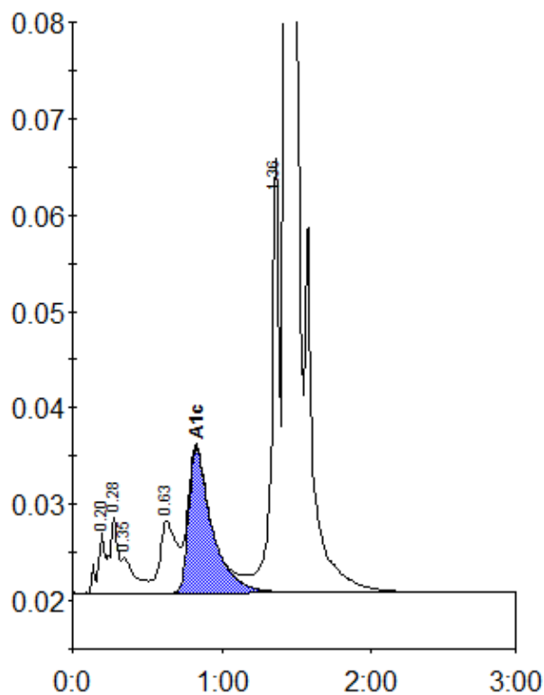
Peak table - ID: 10212851
