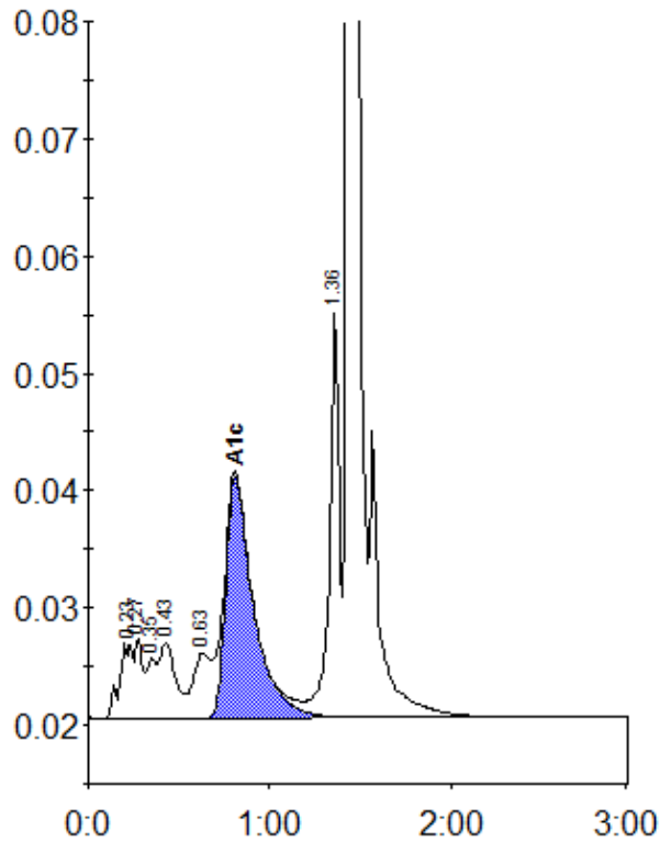
Peak table - ID: 10204715
