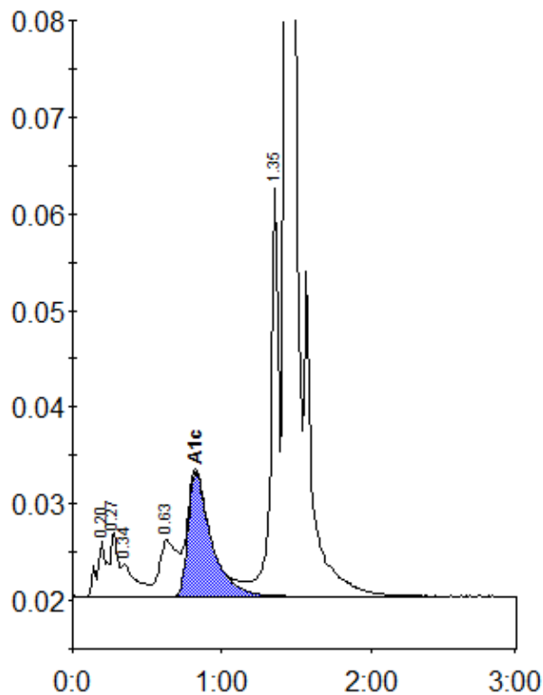
Peak table - ID: 10188644
