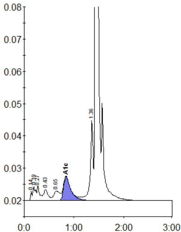
Peak table - ID: 10200337
