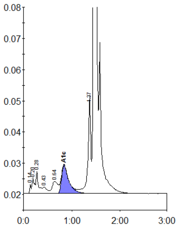
Peak table - ID: 10216200
