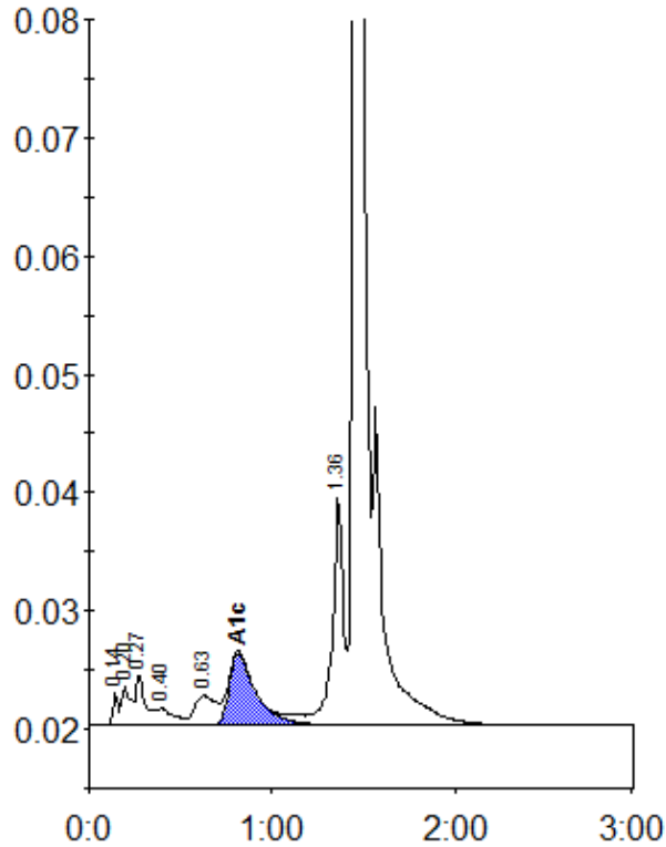
Peak table - ID: 10180809
