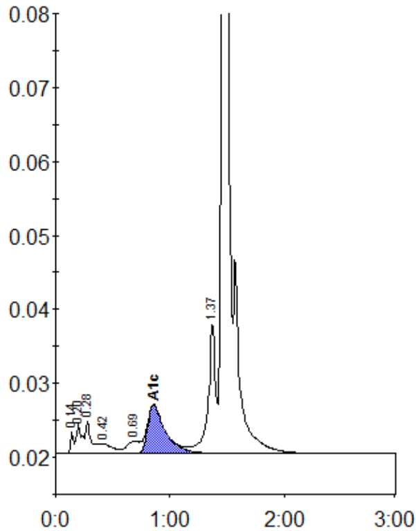
Peak table - ID: 10184496
