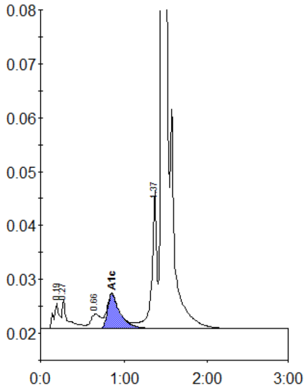
Peak table - ID: 10233068
