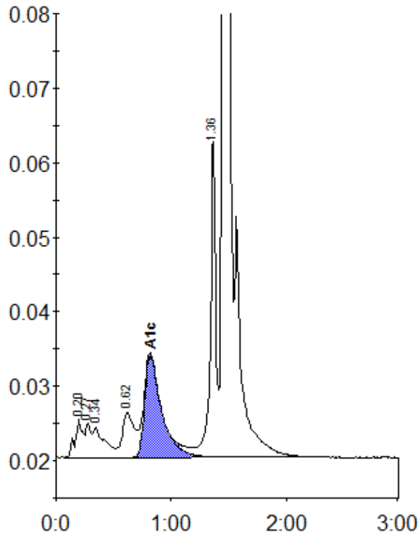
Peak table - ID: 10191317
