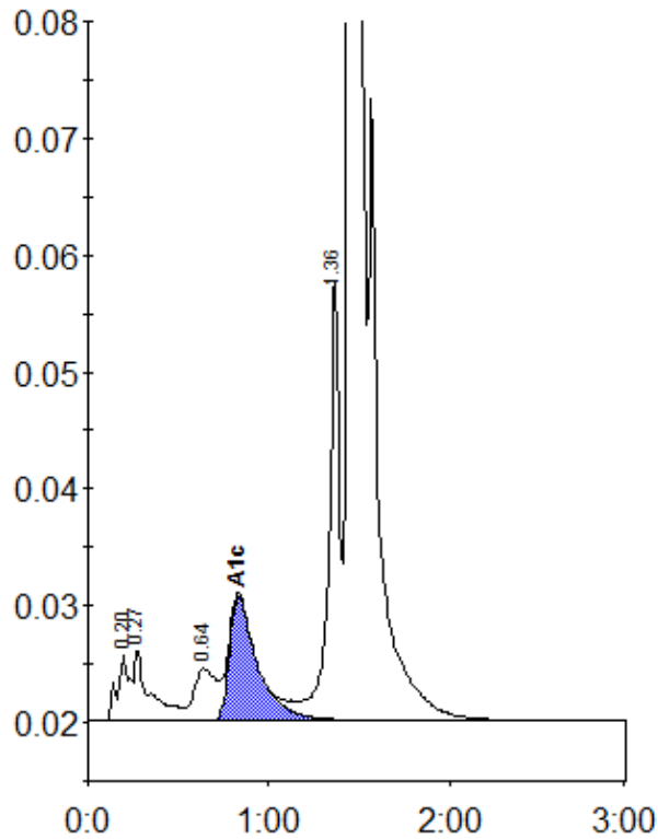
Peak table - ID: 10215564
