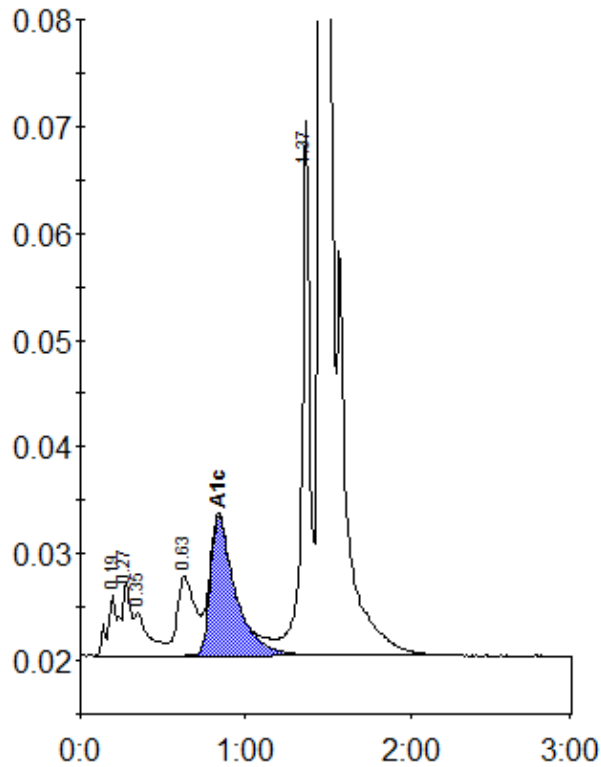
Peak table - ID: 10217048
