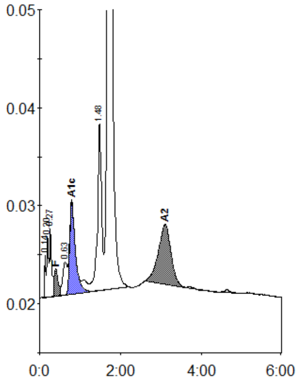
Peak table - ID: 10215342
