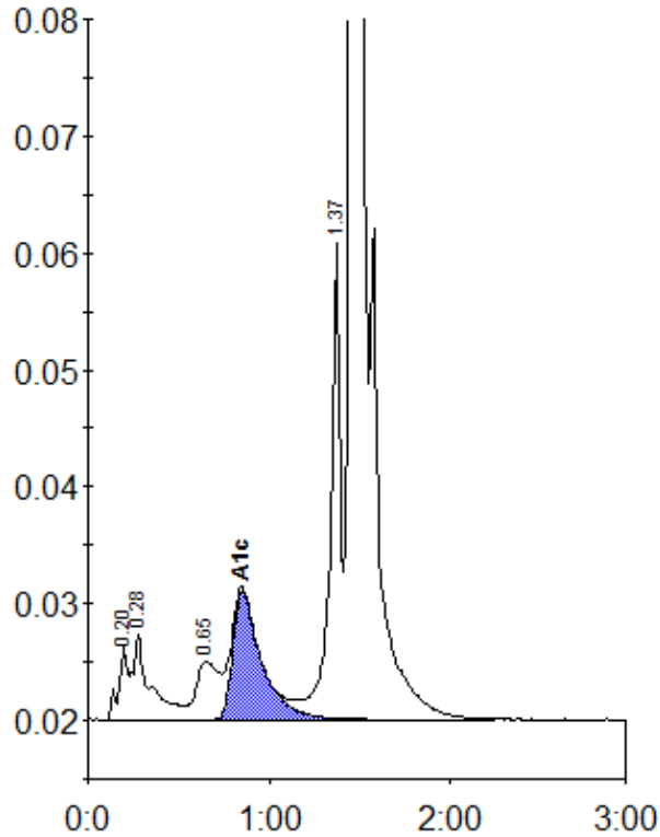
Peak table - ID: 10203449
