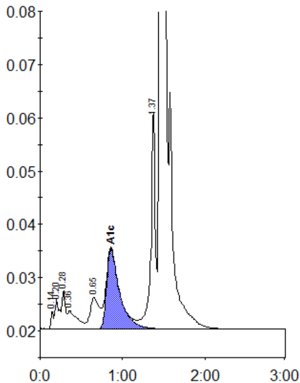
Peak table - ID: 10217594
