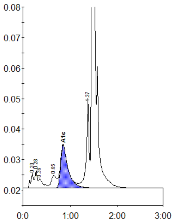
Peak table - ID: 10217599
