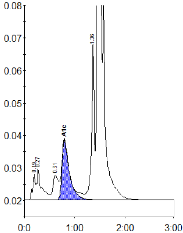
Peak table - ID: 10217650
