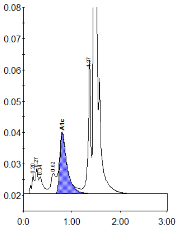
Peak table - ID: 10216641
