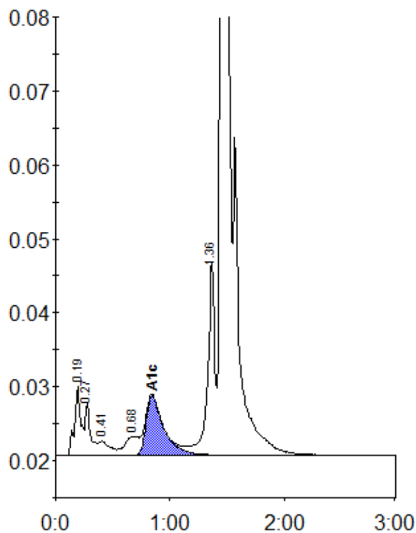
Peak table - ID: 10182762
