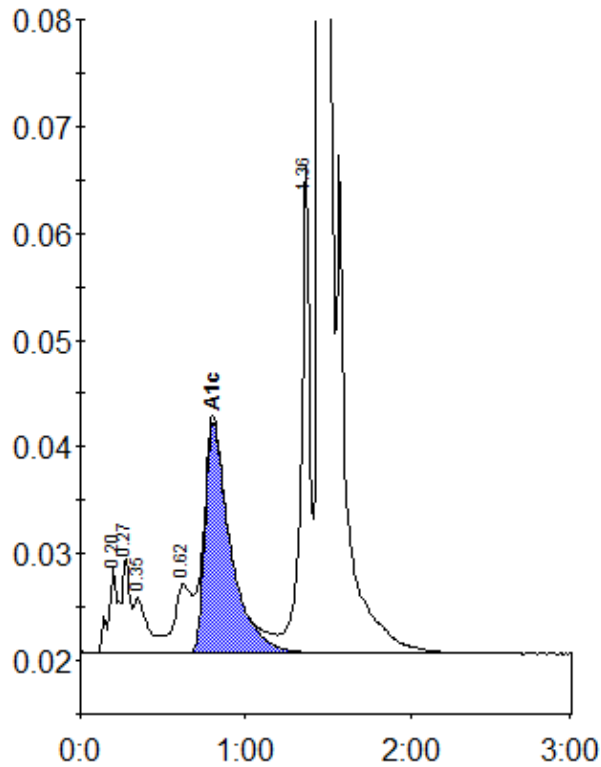
Peak table - ID: 10220732
