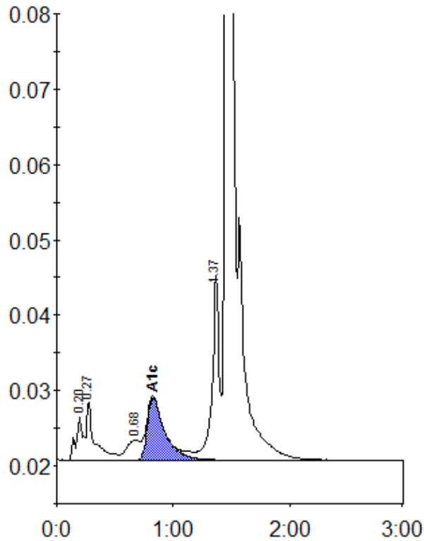
Peak table - ID: 10229238
